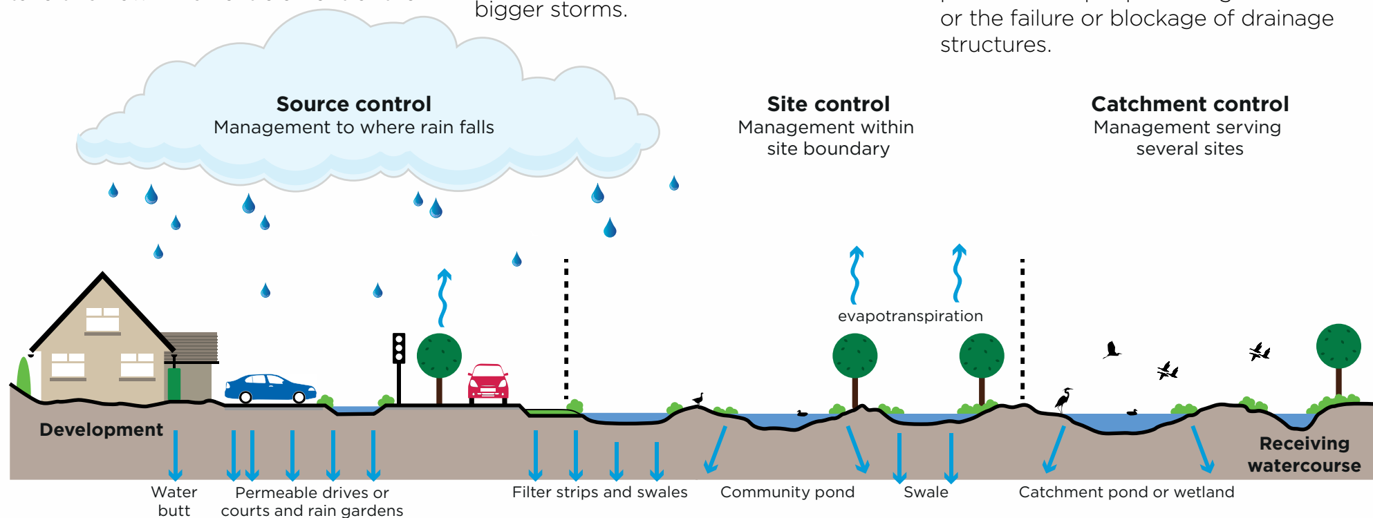
Figure 5: SuDS Management Train (after Sustainable drainage system adoption manual, Anglian Water) 20
