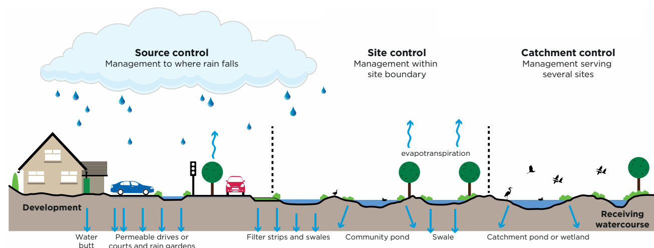
Figure 7: SuDS Management Train (WoE Developers Guide)
