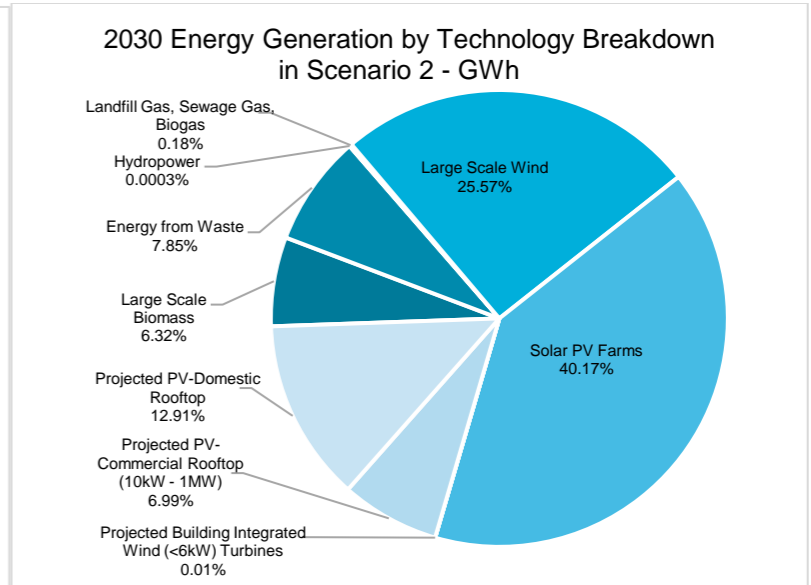
Figure 74: Technology Breakdown of Scenario 2 by GWh
