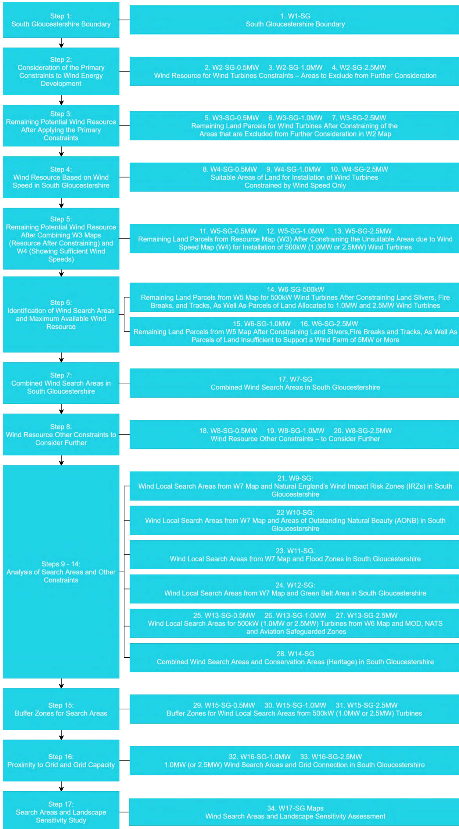
Figure 33: Flowchart of Wind Energy Resource Mapping Process
