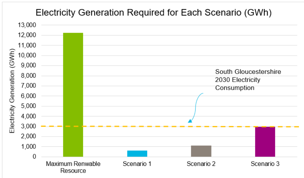
Figure 69: Comparison of Energy Generation Required for Each Scenario
